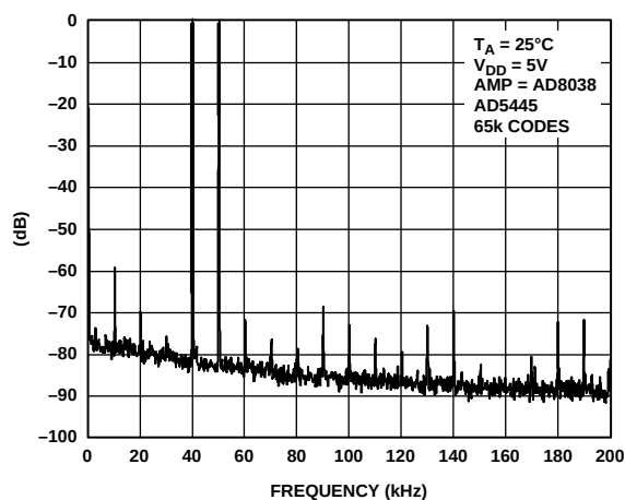
Figure 47. Wideband IMD, f_{OUT} = 60\text{ kHz} , 50\text{ kHz} , Clock = 10\text{ MHz}
