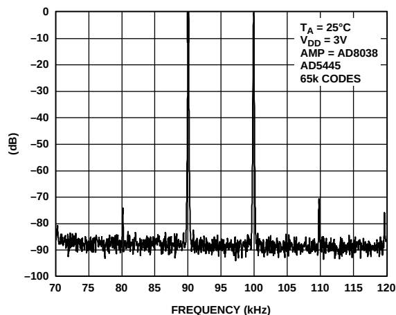
Figure 44. Narrow-Band IMD, f_{OUT} = 90\text{ kHz} , 100 kHz, Clock = 10 MHz
