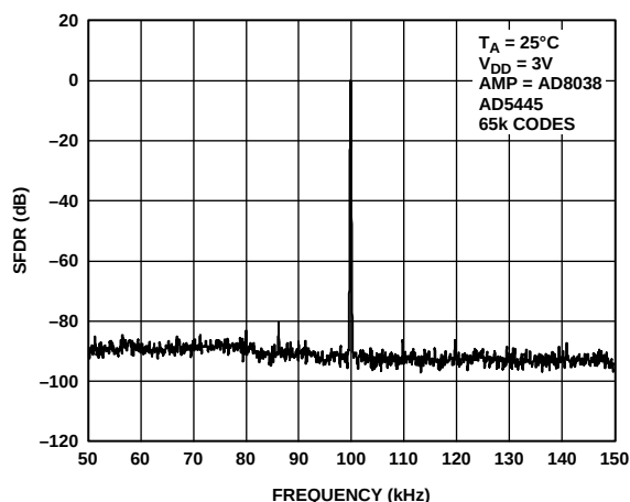
Figure 42. Narrow-Band SFDR, f_{OUT} = 100\text{ kHz} , MCLK = 25 MHz
