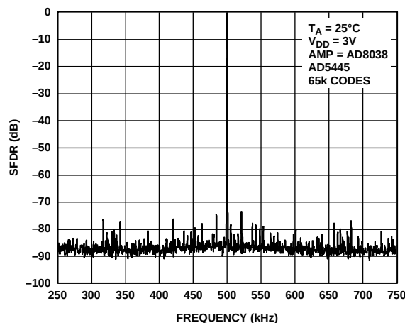
Figure 41. Narrow-Band Spectral Response, f_{OUT} = 500\text{ kHz} , Clock = 25 MHz
