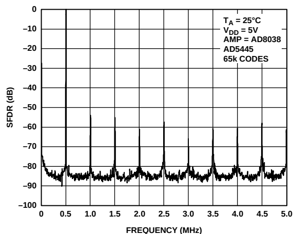
Figure 39. Wideband SFDR, f_{OUT} = 500\text{ kHz} , Clock = 10 MHz
