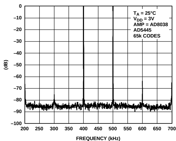
Figure 43. Narrow-Band IMD, f_{OUT} = 400\text{ kHz} , 500 kHz, Clock = 10 MHz
