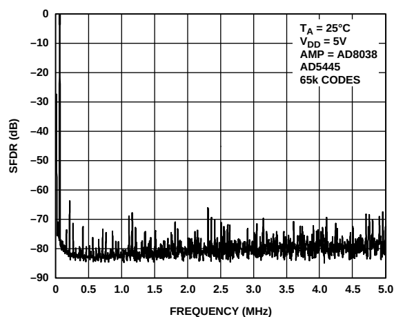
Figure 40. Wideband SFDR, f_{OUT} = 50\text{ kHz} , Clock = 10 MHz
