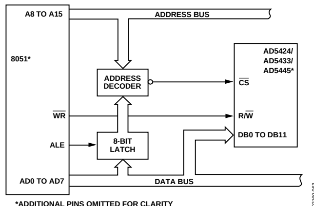
Figure 57. 8xC51-to-AD5424/AD5433/AD5445 Interface
