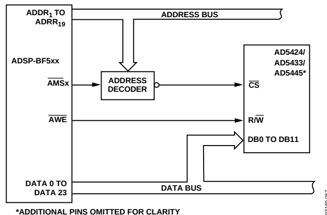
Figure 58. ADSP-BF5xx-to-AD5424/AD5433/AD5445 Interface
