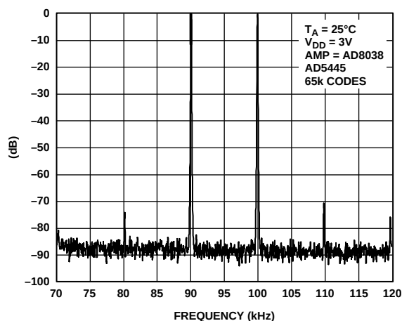
Figure 44. Narrow-Band IMD, f_{OUT} = 90\text{ kHz} , 100 kHz, Clock = 10 MHz
