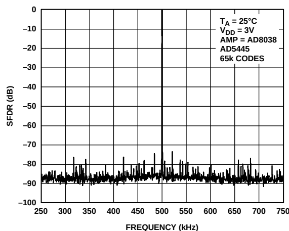
Figure 41. Narrow-Band Spectral Response, f_{OUT} = 500\text{ kHz} , Clock = 25 MHz
