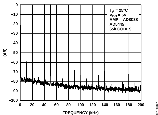
Figure 47. Wideband IMD, f_{OUT} = 60 \text{ kHz} , 50 \text{ kHz} , Clock = 10 MHz
