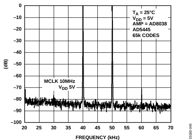
Figure 45. Narrow-Band IMD, f_{OUT} = 40 \text{ kHz} , 50 \text{ kHz} , Clock = 10 MHz
