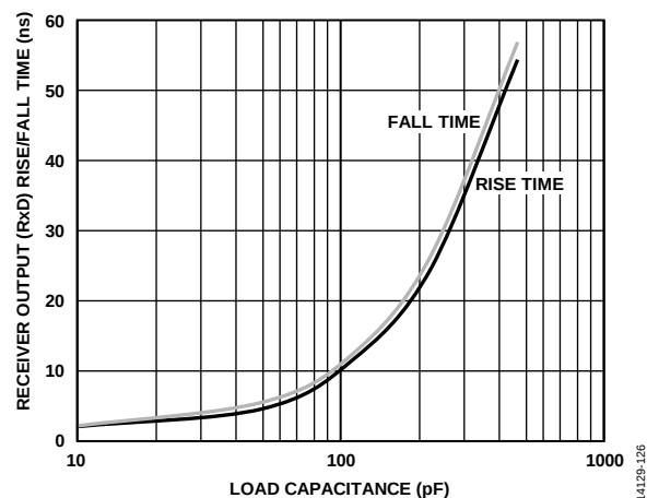
Figure 26. Receiver Output (RxD) Rise/Fall Time vs. Load Capacitance
