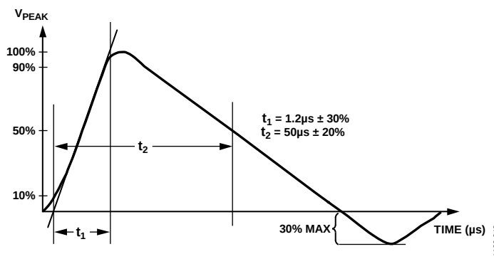
Figure 44. IEC 61000-4-5 Surge 1.2 \mu s/50 \mu s Waveform
