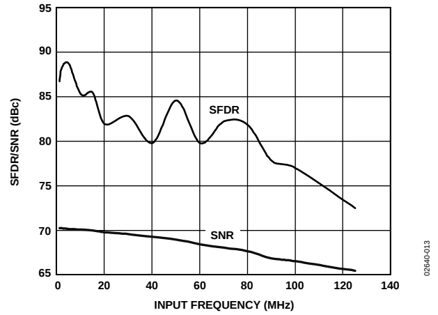
Figure 14. AD9238-65 Single-Tone SNR/SFDR vs. f_{IN}
