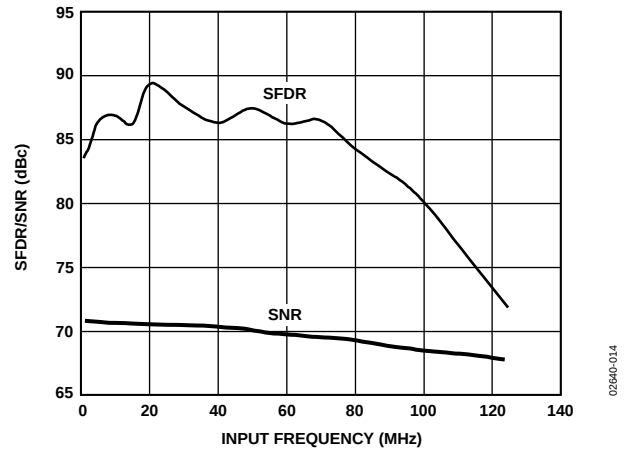
Figure 15. AD9238-40 Single-Tone SNR/SFDR vs. f_{IN}
