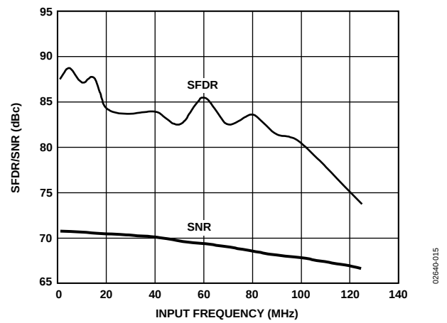
Figure 16. AD9238-20 Single-Tone SNR/SFDR vs. f_{IN}
