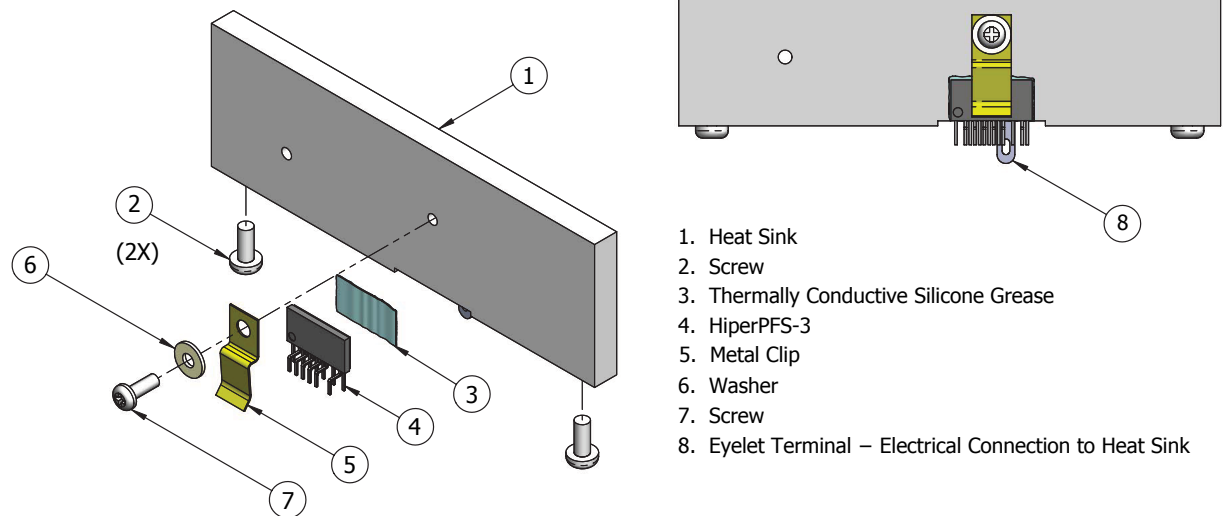
Figure 16. Heat Sink Assembly – with Metal Clip.
