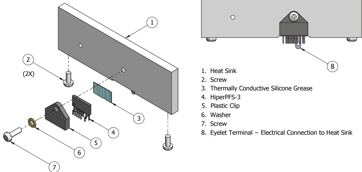
Figure 17. Heat Sink Assembly – with Plastic Clip.
