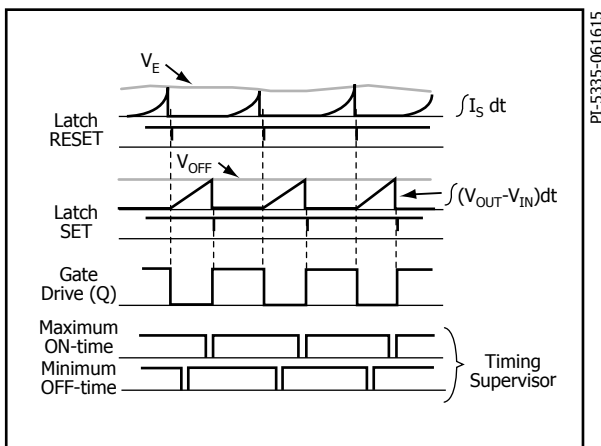
Figure 5. Idealized Converter Waveforms.
