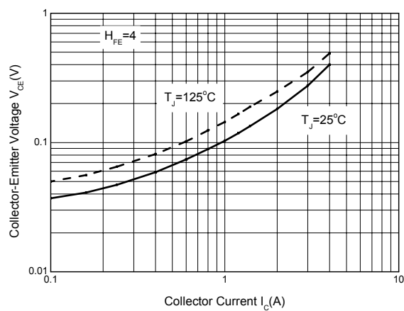
Figure 9. Collector-Emitter Saturation Region
