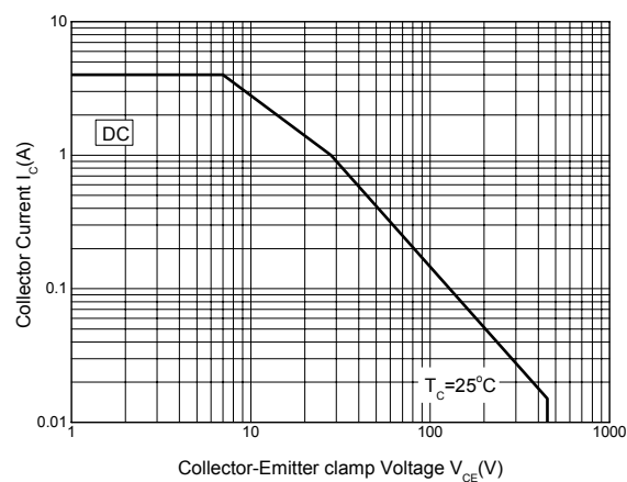
Figure 5. Safe Operating Areas (TO-220F-3 Package)
