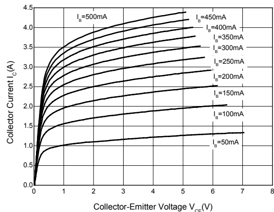
Figure 7. Static Characteristics
