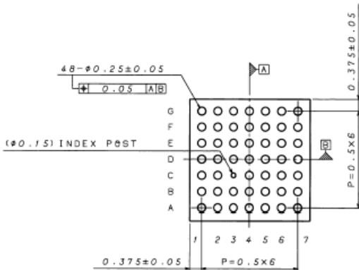
Figure. 64 Package dimensions (UNIT:mm)
