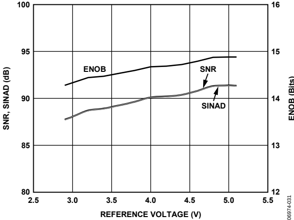
Figure 16. SNR, SINAD, and ENOB vs. Reference Voltage
