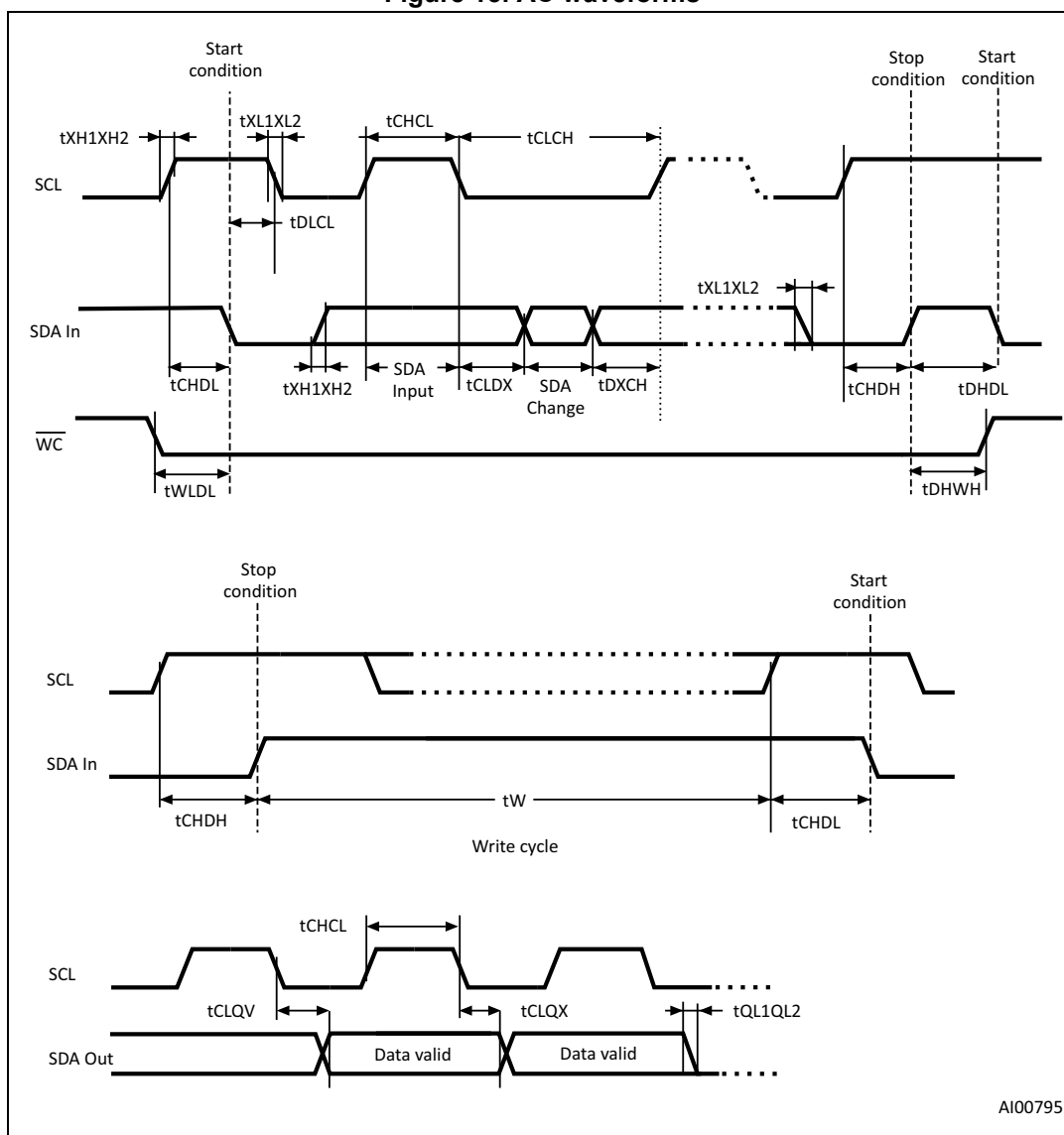
Figure 15. AC waveforms
