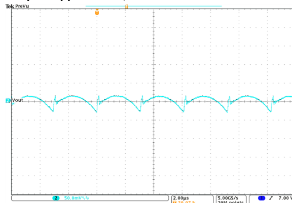
Cout = 8X 100μF Ceramic, Vout = 50mV/Div, 2.0us/Div 331104
