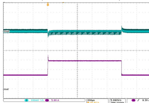
24Vin to 1.0Vout, Cout = 8X 100μF Ceramic Vout (Ch2) = 100mV/Div, Iout (Ch3) = 5A/Div, 200uS/Div 331102
