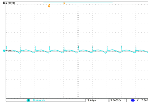
Cout = 8X 100μF Ceramic, Vout = 50mV/Div, 2.0us/Div 331106
