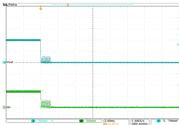
Vout (Ch2) = 500mV/Div, Iin (Ch4) = 500mA/Div, 2ms/Div 331103
