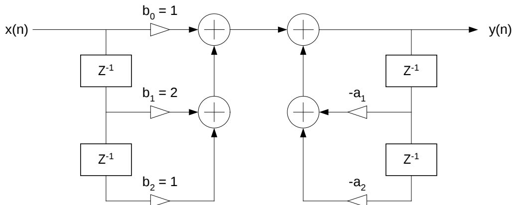
Figure 11 - IIR Diagram
