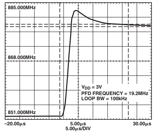
TPC 4. PLL Settling Time, 852 MHz to 878 MHz, 23 μs ( \pm 400 \text{ kHz} )
