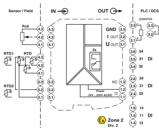
Figure 1 Sensor connection - resistance thermometers and potentiometers
