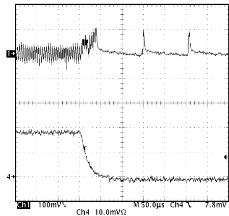
PWM → PSM 3 V Converter (V IN = 10 V)
