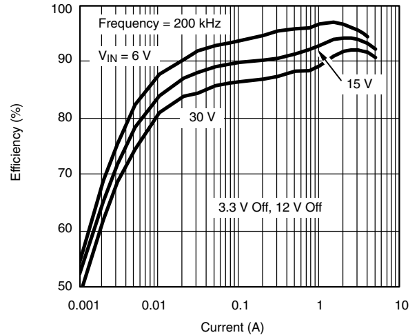
Efficiency vs. 5.0 V Output Current
