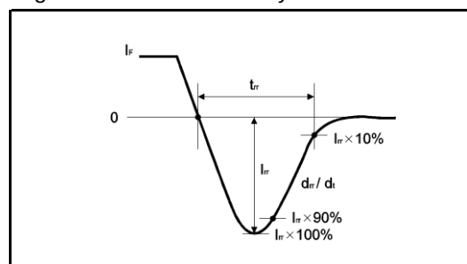
Fig.4-2 Reverse Recovery Waveform
