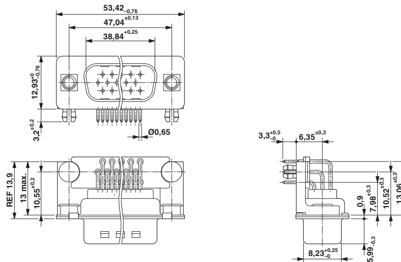
Dimensioned drawing
