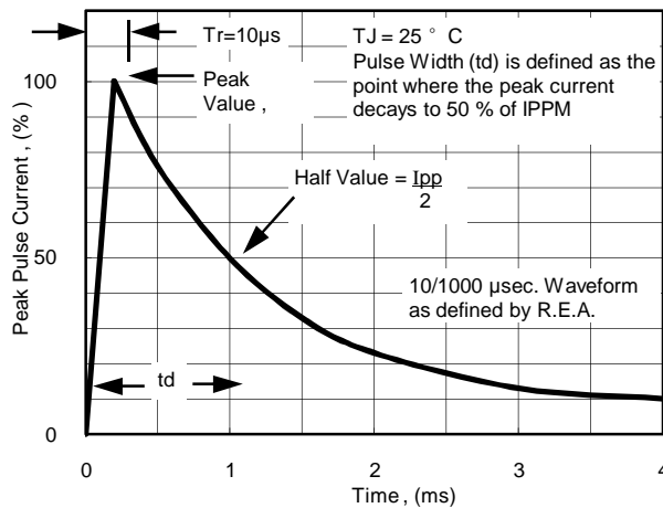
Fig. 4 - Pulse Waveform
