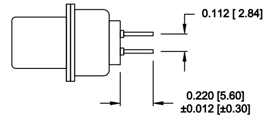
SIGNAL CONTACTS
