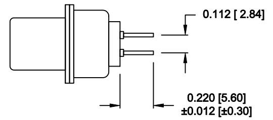
SIGNAL CONTACTS
