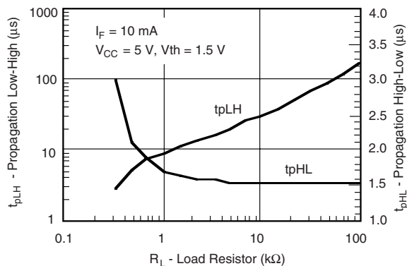
Fig. 17 - -1, Propagation Delay vs. Collector Load Resistor
