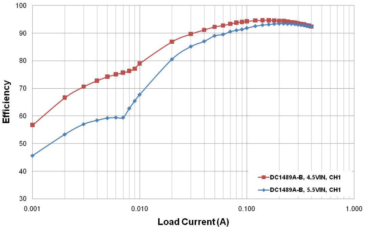
Figure 4. Typical Efficiency vs. Load Current, CH1, 3.3Vout for A-A and A-B boards
