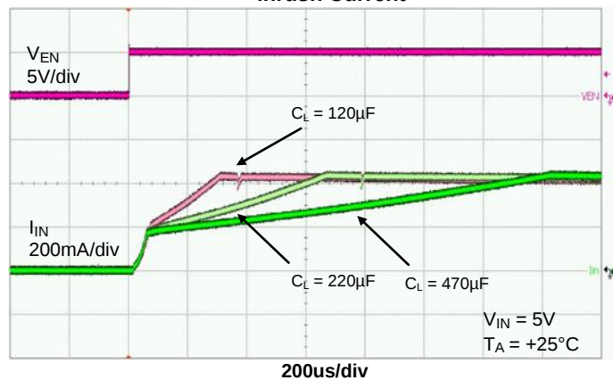
Inrush Current
