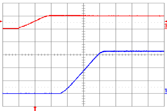
Fig. 3.3V.5: Turn-on transient for V_{out} = 3.3\text{V} with application of V_{in} at full rated load current (resistive) and 47\mu\text{F} external capacitance at V_{in} = 5\text{V} . Top trace: V_{in} (5V/div.); Bottom trace: output voltage (1V/div.); Time scale: 2ms/div.
