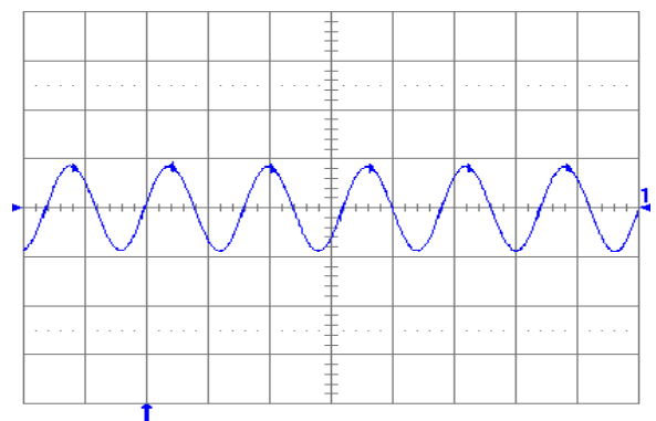
Fig. 3.3V.6: Output voltage ripple (20mV/div.) at full rated load current into a resistive load with external capacitance 47\mu\text{F} ceramic + 1\mu\text{F} ceramic and V_{in} = 5\text{V} for V_{out} = 3.3\text{V} . Time scale: 2µs/div.
