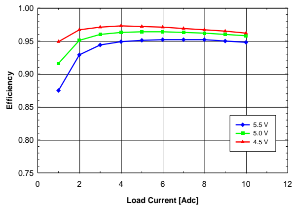
Fig. 3.3V.3: Efficiency vs. load current and input voltage for V_{out} = 3.3\text{V} converter mounted vertically with air flowing from pin 10 to pin 1 at a rate of 200 LFM (1m/s) and T_a = 25^{\circ}\text{C} .
