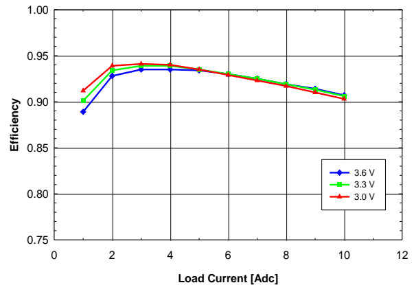
Fig. 1.5V.4: Efficiency vs. load current and input voltage for V_{out} = 1.5V converter mounted horizontally with air flowing from pin 10 to pin 1 at a rate of 200 LFM (1m/s) and T_a = 25^\circ C .
