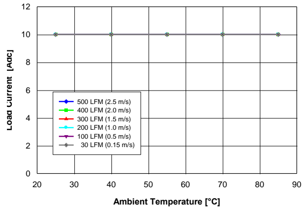
Fig. 3.3V.2: Available load current vs. ambient temperature and airflow rates for V_{out} = 3.3\text{V} converter mounted horizontally with V_{in} = 5\text{V} , air flowing from pin 10 to pin 1, and maximum MOSFET temperature \leq 120^{\circ}\text{C} .
