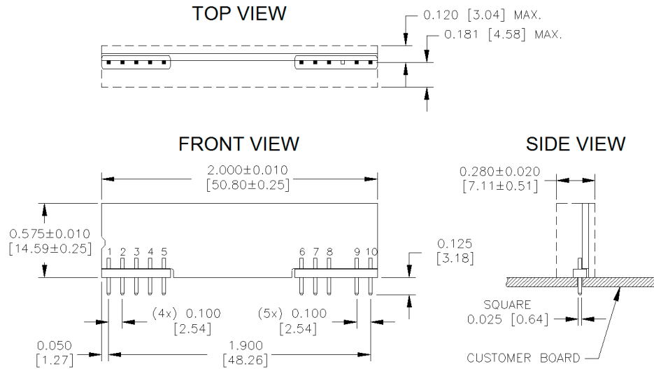
YNV05T10 Pinout (Through-Hole - SIP)
