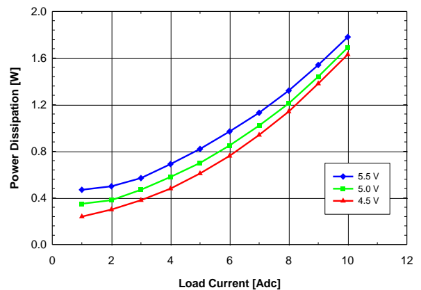
Fig. 3.3V.4: Power loss vs. load current and input voltage for V_{out} = 3.3\text{V} converter mounted vertically with air flowing from pin 10 to pin 1 at a rate of 200 LFM (1m/s) and T_a = 25^{\circ}\text{C} .
