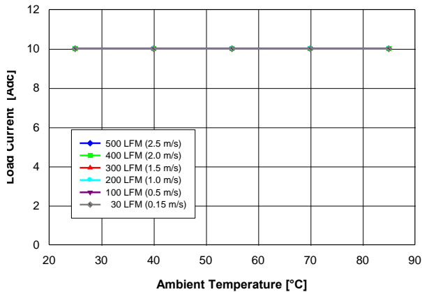
Fig. 3.3V.1: Available load current vs. ambient temperature and airflow rates for V_{out} = 3.3\text{V} converter mounted vertically with V_{in} = 5\text{V} , air flowing from pin 10 to pin 1, and maximum MOSFET temperature \leq 120^{\circ}\text{C} .
