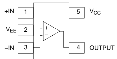
STYLE 3 PINOUT
