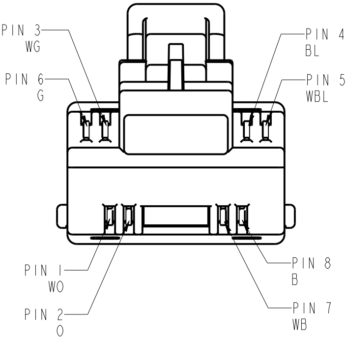
RIGHT PLUG WIRING DIAGRAM
