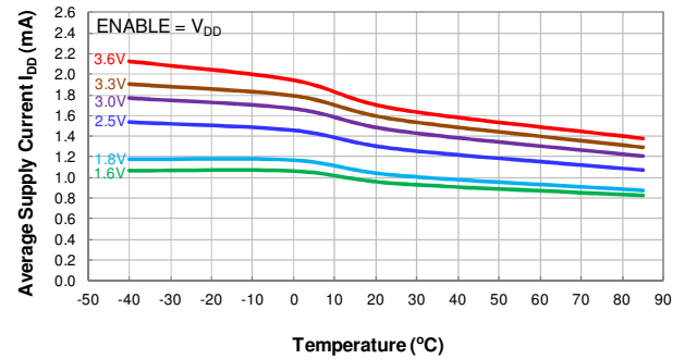
Average Supply Current (ENABLE = V_{DD} ) vs Temperature
