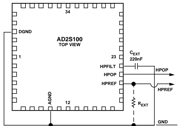
Figure 6. AD2S100 Homopolar Output Connections
