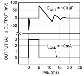
MIC2930x Load Transient
