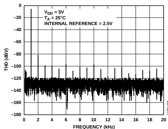
Figure 49. Total Harmonic Distortion (THD) at 1 kHz
