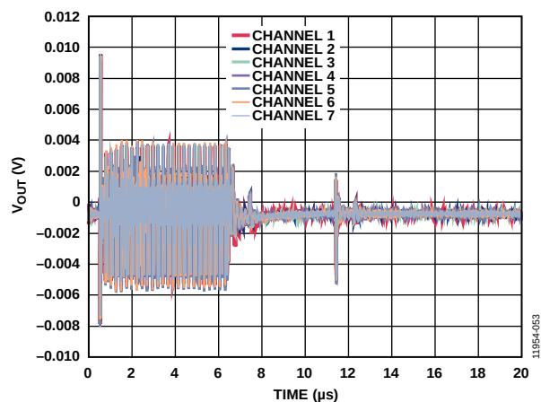
Figure 46. DAC-to-DAC Crosstalk
