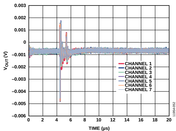
Figure 45. Analog Crosstalk
