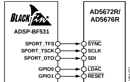
Figure 70. SPORT Interface
