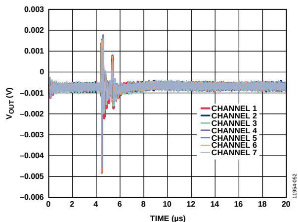
Figure 45. Analog Crosstalk
