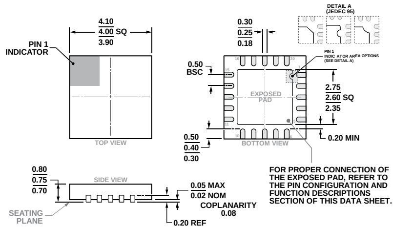
Figure 74. 20-Lead Lead Frame Chip Scale Package [LFCSP] 4 mm × 4 mm Body and 0.75 mm Package Height (CP-20-8) Dimensions shown in millimeters
