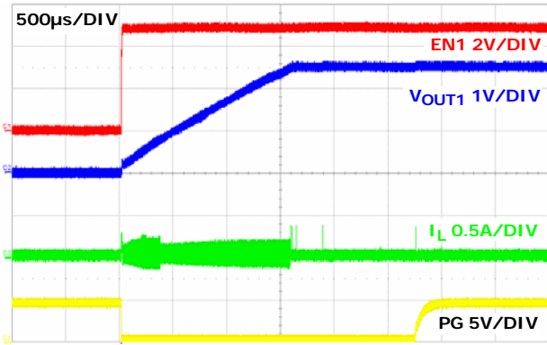
FIGURE 26. SOFT-START AT NO LOAD CHANNEL 1 (PFM)
