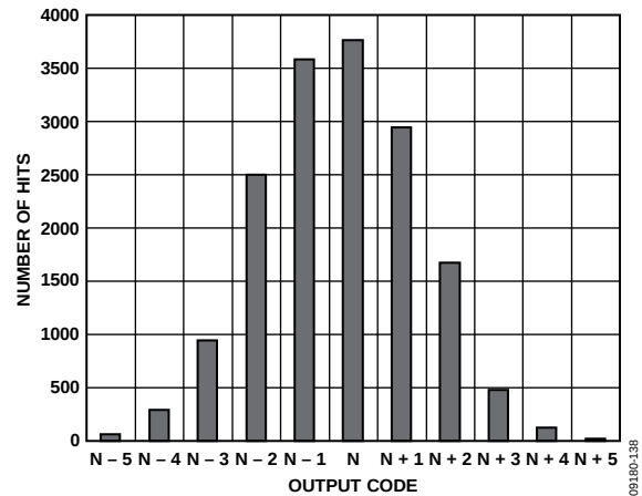
Figure 38. AD9644-155 Grounded Input Histogram
