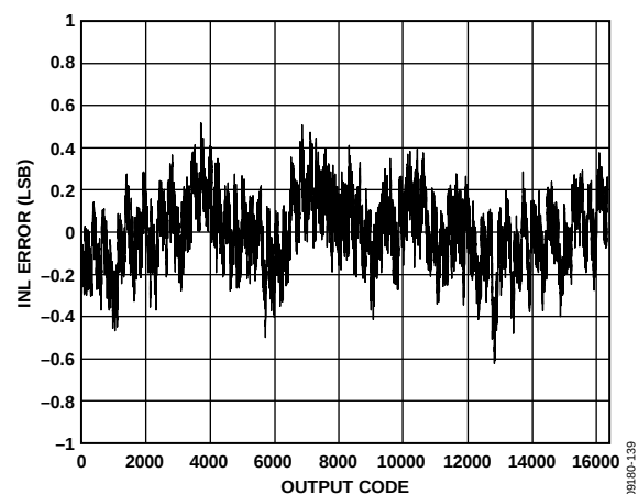
Figure 39. AD9644-155 INL with f_{IN} = 30.3 MHz
