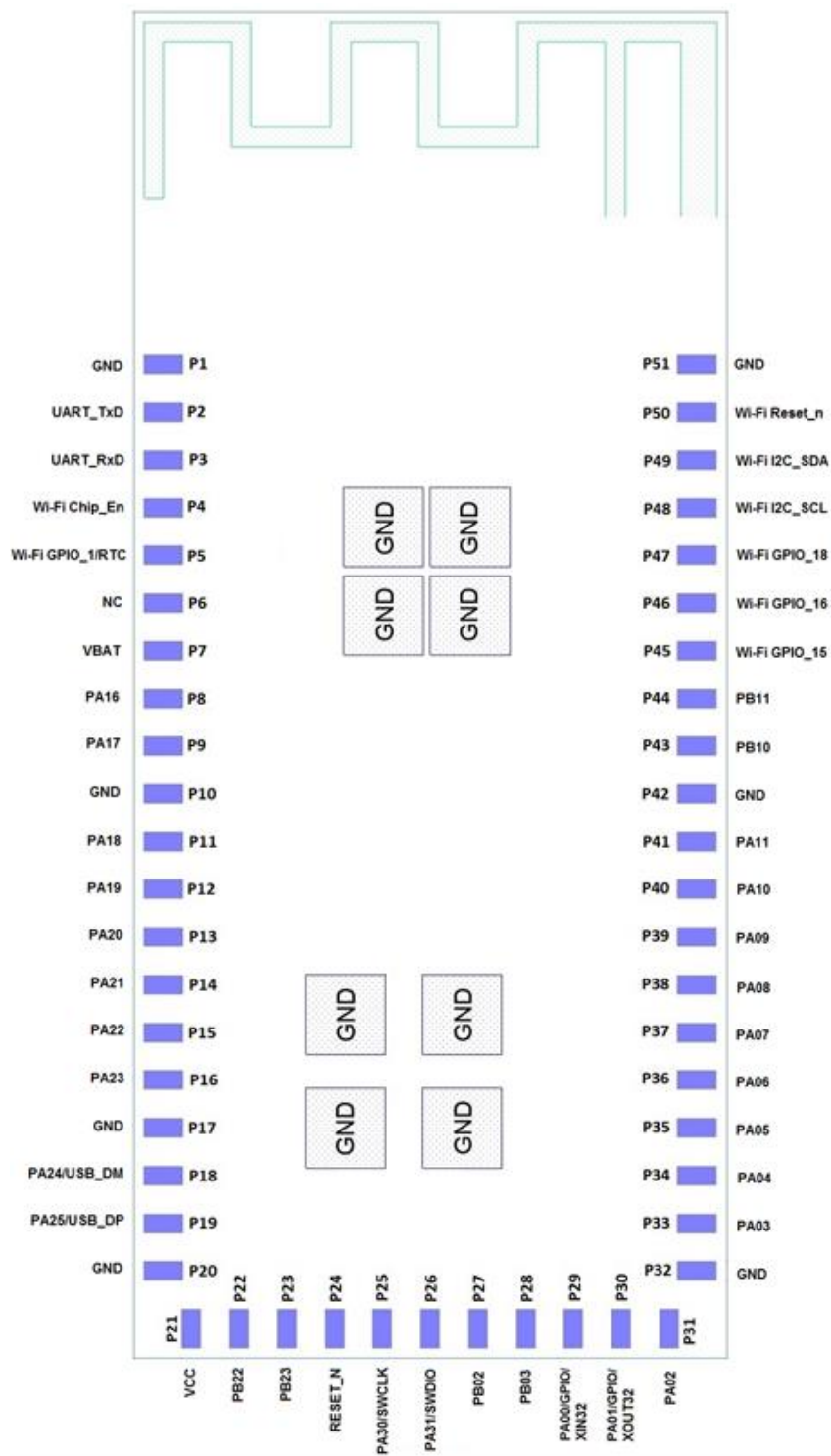
Figure 3-1. Pin Assignment
