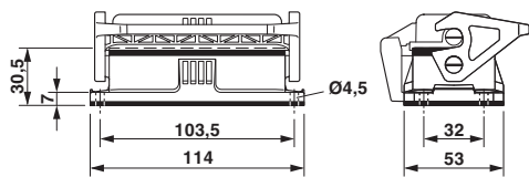
Dimensional drawing
