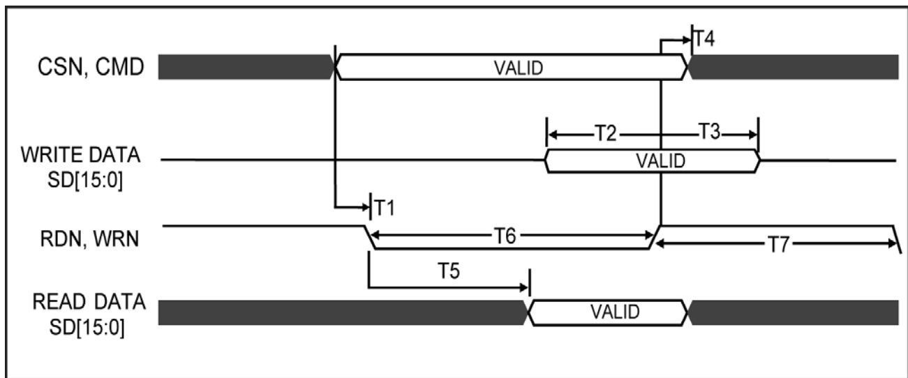
Figure 11. Asynchronous Cycle
