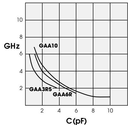
Self-Resonant Freq. vs. Capacitance
