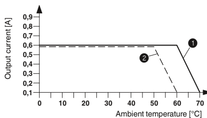
Derating curve ELR H3-IES-SC-230AC/500AC-0,6 100% operating time
