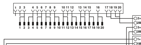
Connection scheme FLKM 50-PA-S300/SO167
