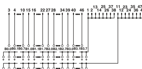
UM 45-FLK50/32IM/ZFKDS/PLC connection scheme
