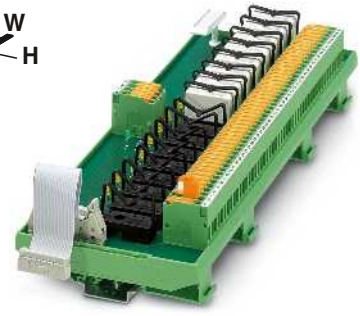
Output extension module for 16 miniature relays with knife/disconnect terminal blocks, 1 PDT
