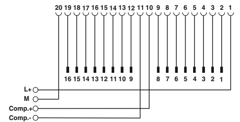
FLKM 16-PA-S300/MINI-MCR connection scheme
