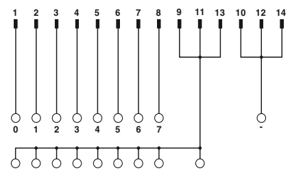
Connection scheme VIP-2/.../FLK14/8P/PLC
