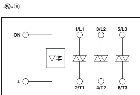
For switching 3~ AC motors up to 575 V AC/3 x 16 A
