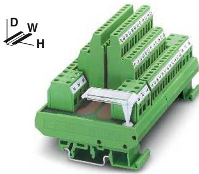
With screw connection and 6 potential levels
