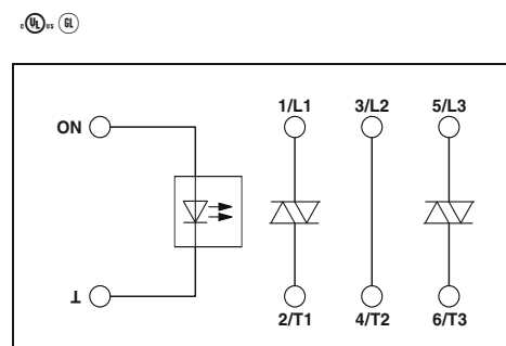
For switching 3~ AC motors up to 575 V AC/3 x 37 A
