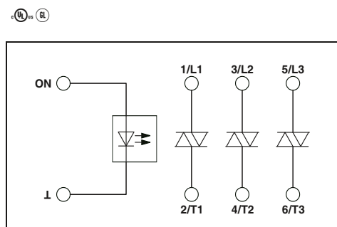
For switching 3~ AC motors up to 575 V AC/3 x 9 A
