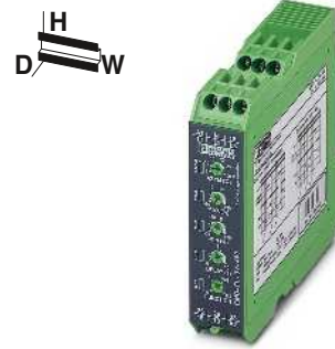
Undervoltage and phase monitoring, 400 V or 230 V
