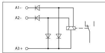
Block diagram of a bistable relay, negative switching type
