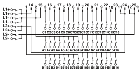
FLKM-D25 SUB/B/KDS3-MT/TU830 connection scheme
