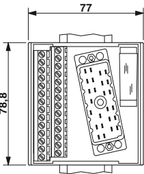
Dimensional drawing for UMK-EC56/25/EX-R
