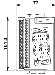
Dimensional drawing for UMK-EC90/32/EX-XUR
