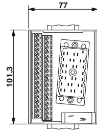
Dimensional drawing for UMK-EC90/32/EX-XOR
